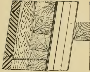
'Warrior' (England) 1859. Side Armor Iron 4 1/2 in. Solid.
